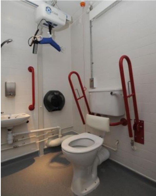
OT200 Ceiling Hoist on H frame system giving hoist access to the WC, Changing Table and transfer area
